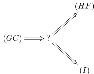
Figure 3: Is there a physically significant intermediate condition which is implied by (GC) and implies both (HF) and (I)?
