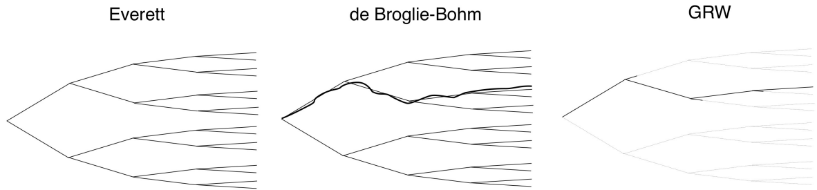
Figure 4: The Everett, de Broglie-Bohm and GRW interpretations of quantum mechanics all rely on the branching structure generated through decoherence in order to recover the phenomenology of wave function collapse (assuming, that is, that their collapse mechanisms are decoherence-compatible). According to Everett’s interpretation, no modifications to the quantum state or Schrodinger dynamics are necessary to recover the phenomenology of collapse. According to the dBB interpretation, an additional configuration (whose trajectory is represented by the thick black curve in the middle diagram) singles out one branch as dynamically and phenomenologically relevant; all other branches continue to exist, but are irrelevant to the configuration’s trajectory and to the theory’s phenomenology. Assuming that the GRW collapse mechanism is decoherence-compatible, the unitary branching structure represents the set of all possible stochastic state evolutions on GRW theory; while only one such evolution occurs (bold line in the right-hand figure), the unrealized branches (represented by the dotted lines in the right-hand figure) may be interpreted as evolutions that could have occurred on this evolution.
