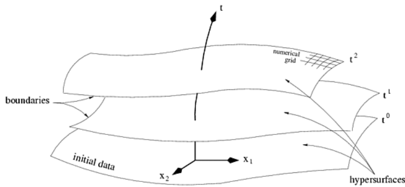
Fig. 1 A ‘presentist-friendly’ space-time: Evolving 3-dimensional space-like surfaces in a space-time with a preferred time-direction.
