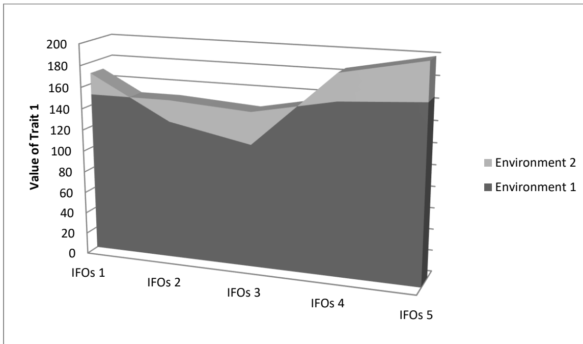
Figure 1. Contributions of two different environments to a trait value as a function of IFOs. The innate range of the trait for IFOs 1 is 150-170. The innate range of the trait for Environment 1 is 145-165.
