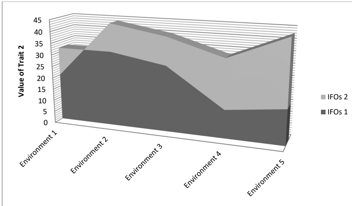
Figure 2. Contributions of two different IFOs to a trait value as a function of environment. The innate range of the trait for environment 1 is 20-32. The innate range of the trait for IFOs 1 is 15-32.
