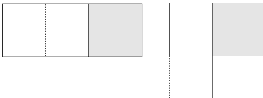
Figure 1. Cut-and-paste manipulations in the procedure BM 13901 #1. The sides of the square are a bit larger in the drawing in relation to the rectangle when taking into account the calculated result.
