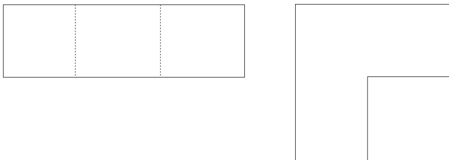
Figure 2. Cut-and-paste manipulations in the procedure YBC 4663#8.
