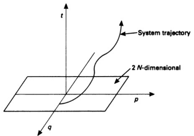
Fig. 2 The extended phase space.
