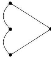
Fig. 3: An example of Eulerian graph
