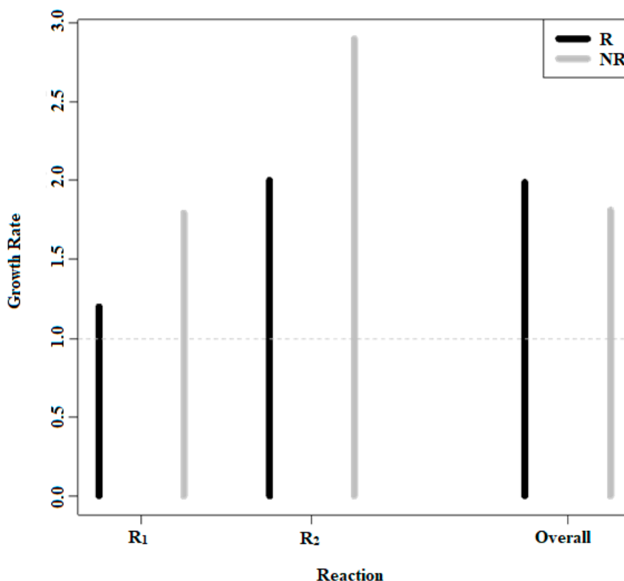
Figure 2. From Table 3 is visually represented. The “dark” line represents “R” (ribose) and the “grey” line represents “NR” (non-ribose). Although the dark lines in R 1 and R 2 are shorter than the grey lines, in the overall population, the dark line dominates over the grey line. This reversal allows us to jettison the inefficiency objection to the RWT.
