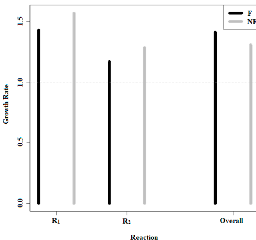
Figure 1. From Table 2 is visually represented. The “dark” line represents “F” (acetyl-CoA) and the “grey” line represents “NF” (non-functional molecules). Even though in R 1 and R 2 , the dark lines are shorter in length than the grey lines, in the overall population, the former dominate over the latter showing the required reversal to reject the inefficiency objection to the MFT.
