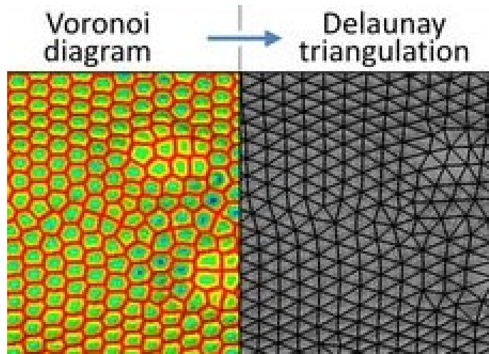
Figure 3: Voronoi tiling diagrams and Delaunay triangulation from Manukyan et al. (2017).
