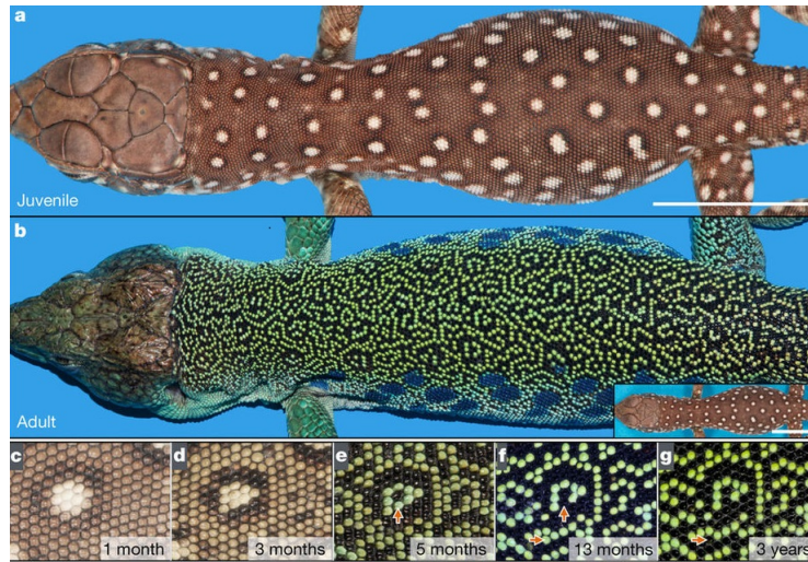
Figure 2: Change in the skin color patterns of ocellated lizards from Manukyan et al. (2017).
