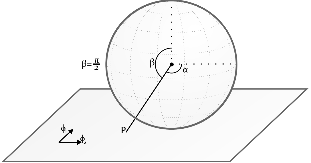
Figure 1: The projection from the \phi_1 - \phi_2 plane onto the sphere in \alpha, \beta . The singularity of general relativity is at \beta = \pi/2 which is a regular point of the equations of motion on the sphere.
