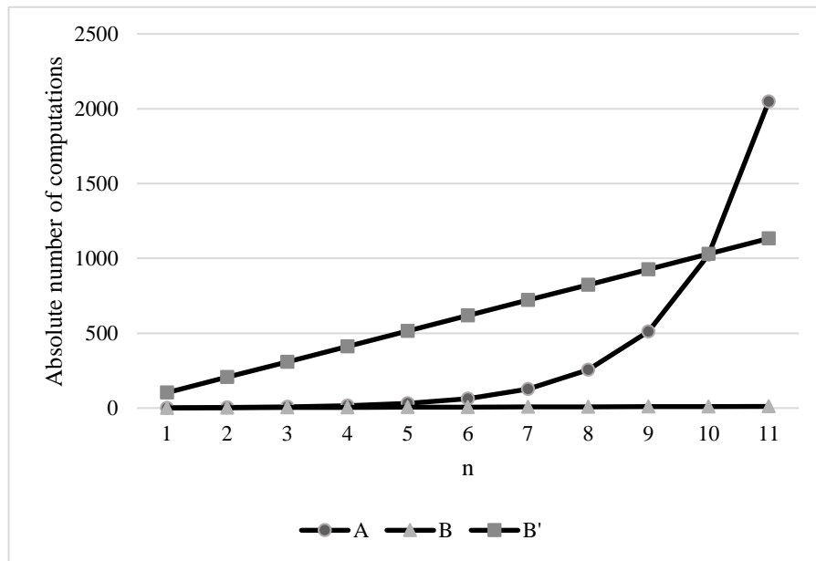
Figure 4 Comparison of the absolute number of computations in three algorithms. B and B' have the same time complexity.
