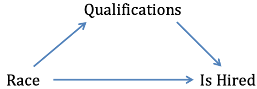
Figure 1: Discrimination DAG
