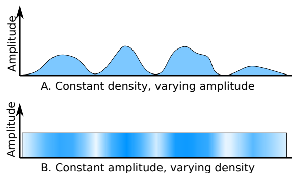
FIG. 2. The Born rule from counting space-states. A. The usual interpretation of a wavefunction as a linear combination of basis state vectors of different norms. B. The interpretation of the wavefunction in terms of constant norm basis state vectors, but with inhomogeneous density.
