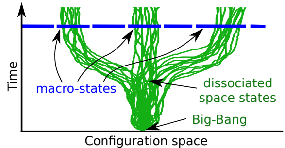
FIG. 1. Wavefunctional dissociation due to quantum-gravitational background freedom. The micro-states (in green) are space-states. They are very similar at the Big-Bang, then background freedom makes them dissociate and form a branching structure like in the many-worlds interpretation. The dissociation is reversible at micro scales, allowing interference, but it becomes irreversible when it manifests at macro scales. The branching structure (in yellow) corresponds to the macro-states (in blue). The distribution of space-states per macro-state or branch gives the Born rule.
