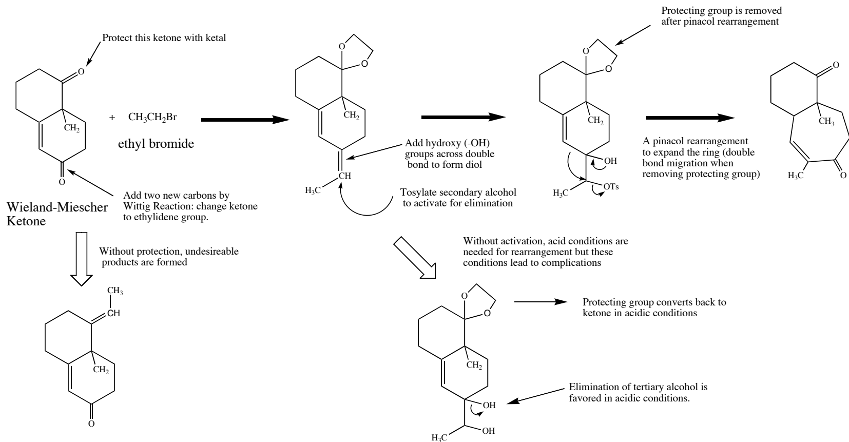
Figure 4: Control steps in the synthesis of longifolene. The black arrows sketch (part of) the actual synthetic path, while the broad arrows indicate what would have happened without the appropriate control.
