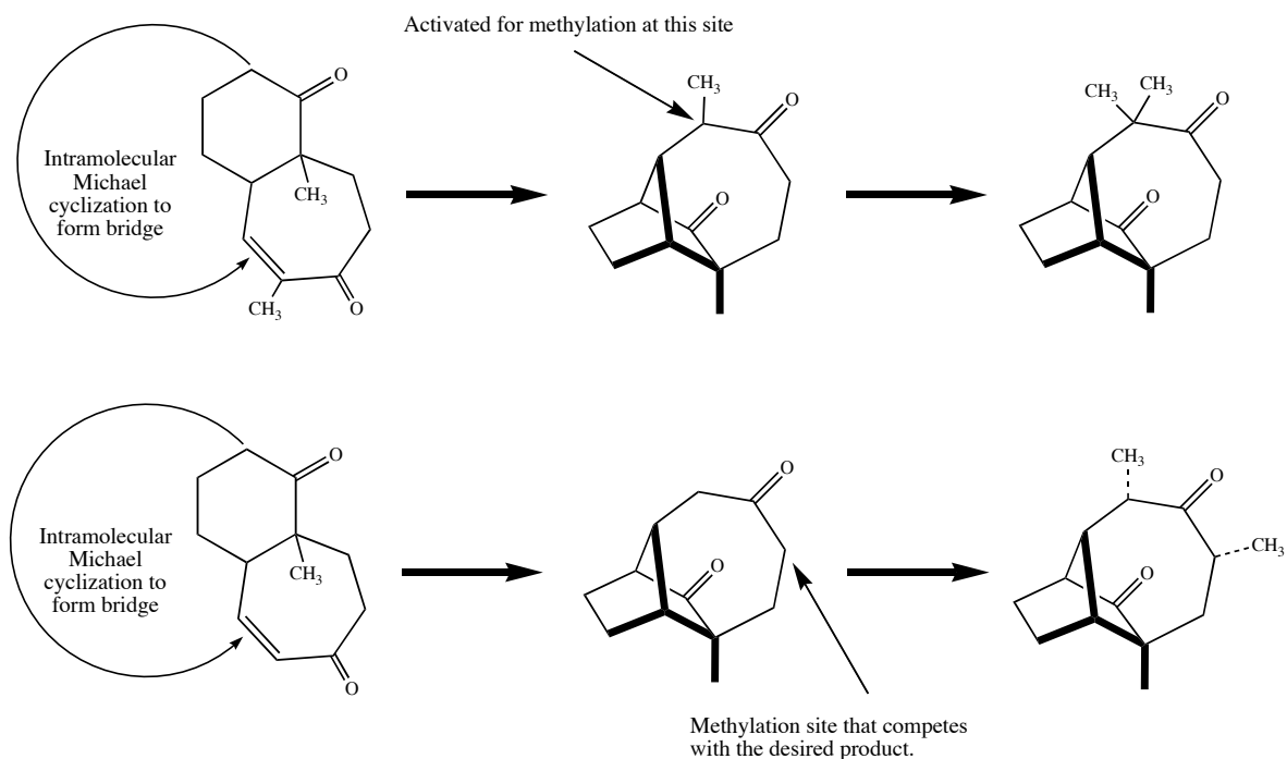
Figure 3: Plausibility assessment in the synthesis of Longifolene. The top path is to be preferred because the product of the intramolecular Michael cyclization is activated for the addition of a methyl group in the correct position. In the bottom path, there are two competing sites for the subsequent addition of the methyl group.
