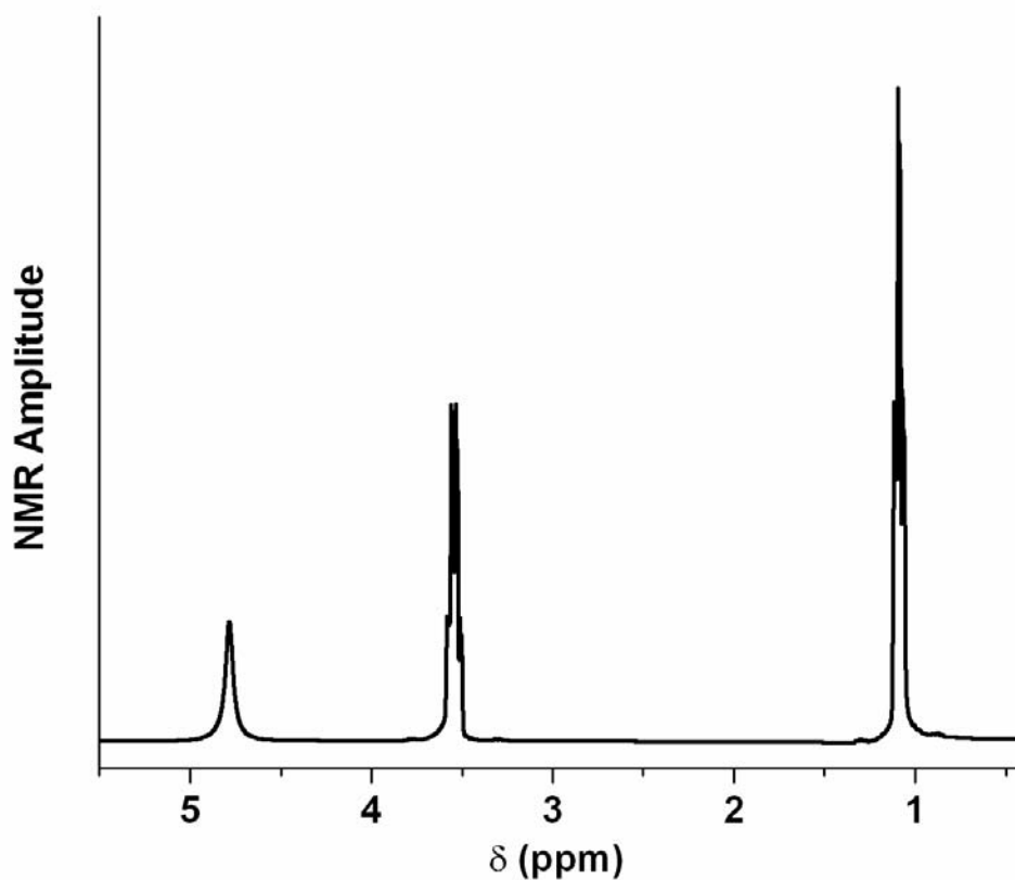
Figure 1 The proton nuclear magnetic resonance (NMR) spectrum of ethyl alcohol ( \text{CH}_3\text{CH}_2\text{OH} ) dissolved in deuterium oxide ( \text{D}_2\text{O} ), showing a clear separation of signals corresponding to reorientation (with respect to an external
