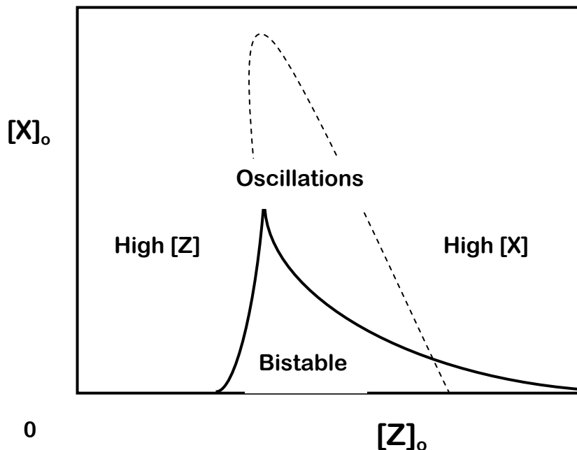
Figure 2 ‘Bifurcation diagram’ (for specific values of k_0 , k , and k' ) for a model of a basic type of oscillating reaction that is shown in Scheme II. On the left, a non-equilibrium steady-state that resembles the reactants (high Z concentration) is stable. On the right, a steady state that resembles the products (high X concentration) is stable. In the center of the figure (within the dotted curve) both steady states are unstable, and continual oscillations occur. In the region labeled ‘bistable’ both steady states are stable — the system may be in either state, depending on its history. Redrawn after Schreiber et al 2003.
