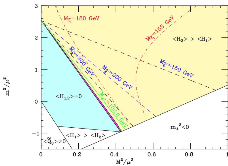
Figure 2: Phase diagram of a minimal supersymmetric model with universal scalar mass m , unified gaugino mass M and Higgsino mass \mu at the GUT scale [47].
