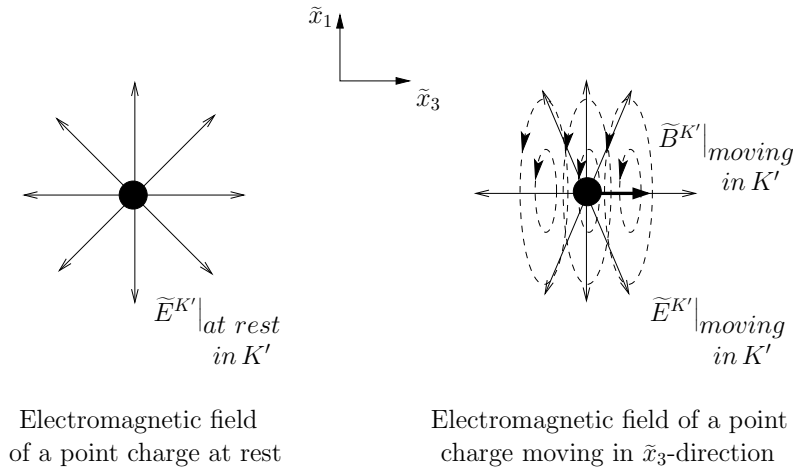
Figure 2: The change of the electromagnetic field of a point charge
