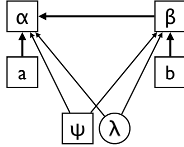
Fig. 3: Direct cause structure
