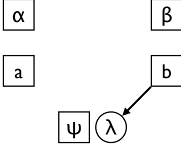
Fig. 25: Violation of Causal Autonomy
