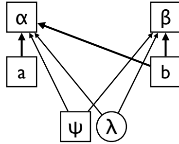
Minimal structures which can violate Bell inequalities (according to the standard Bell argument)
