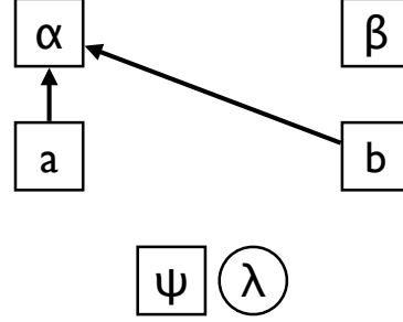
Fig. 26: Violation of No Causal Bell Contextuality 1
