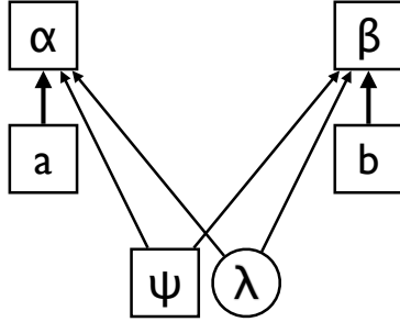
Fig. 12: Local causal structure with hidden variable \lambda
