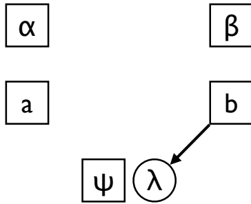
Fig. 16: Violation of Causal Autonomy
