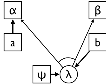
Fig. 37: Structure 36 in the usual variable scheme
