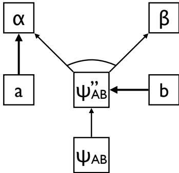
Fig. 36: Reduced causal structure according to quantum mechanics
