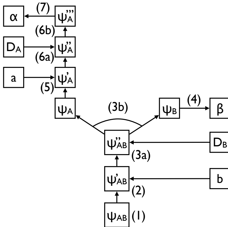
Fig. 33: Detailed causal structure according to quantum mechanics
