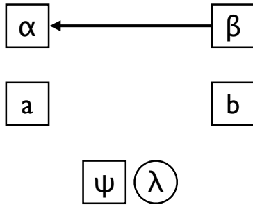
Fig. 14: Violation of Causal Outcome Independence
