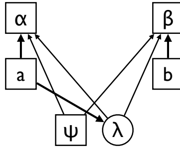
Fig. 22: Non-local structure implying Local Factorisation
