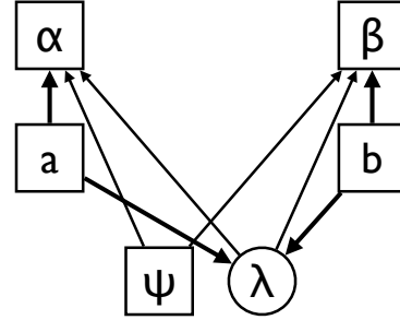
Fig. 13: Non-local causal structure with the hidden variable as common effect of the settings.
