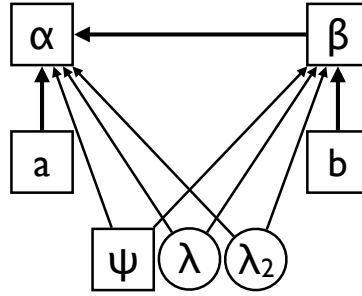
Fig. 31: Direct structure with a second hidden common cause \lambda_2 of the outcomes
