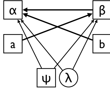
Fig. 24: Direct cause structure 2
