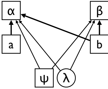
Fig. 4: Non-local common cause structure
