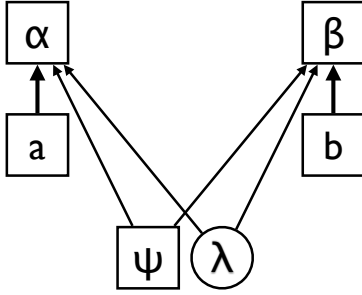
Fig. 2: Local common cause structure
