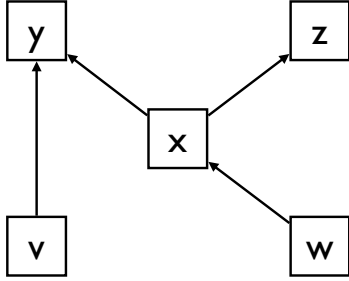
Fig. 34: Example of a causal structure
