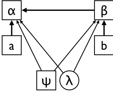
Fig. 23: Direct cause structure 1
