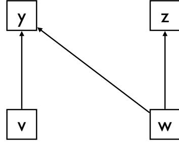
Fig. 35: Eliminating variable x from structure 34
