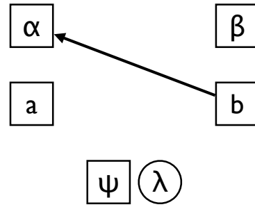
Fig. 15: Violation of Causal Parameter Independence
