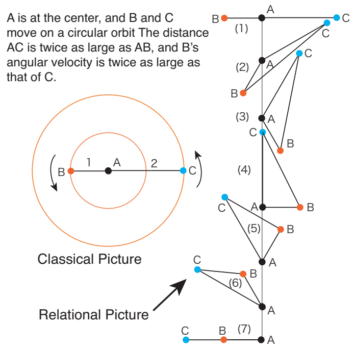
Figure 19: Two Representations of Planetary Motion
