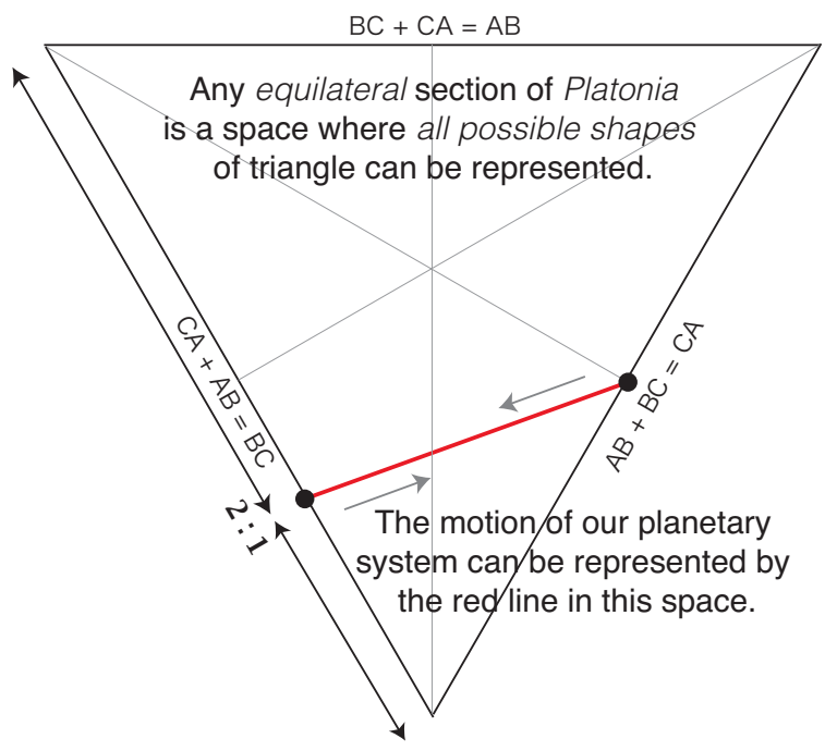
Figure 20: Shape Space and the Planetary Motion
