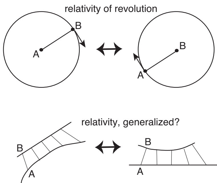
Figure 16: Can Relativity be Generalized?
