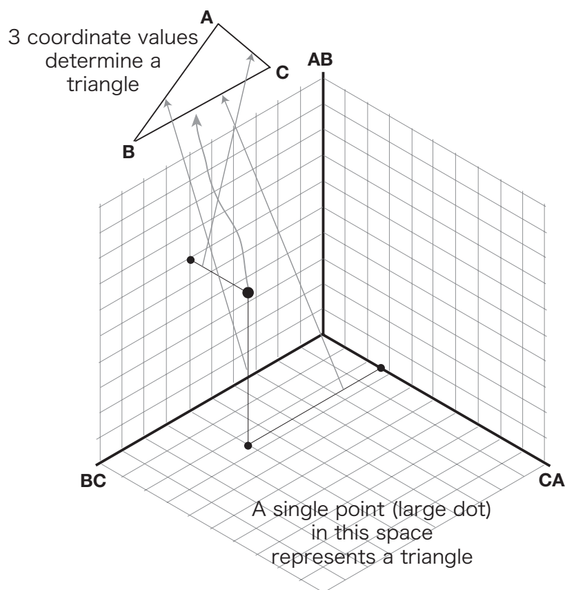
Figure 17: A Configuration Space
