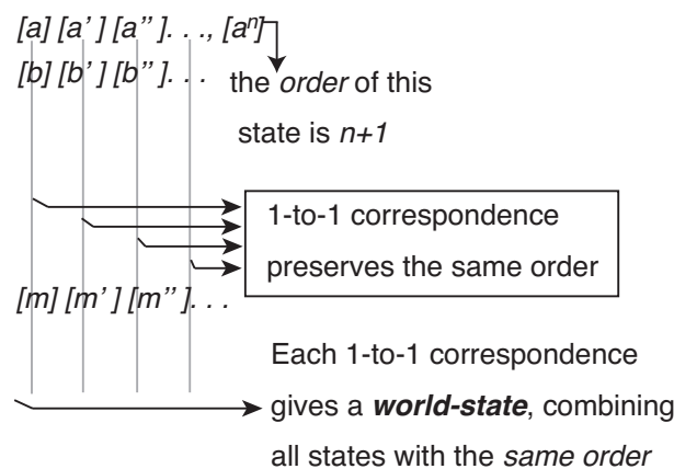
Figure 11: World-States by 1-to-1 Correspondence
