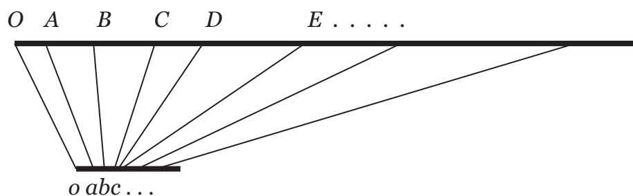
Figure 12. Alignment of States between two Continua
