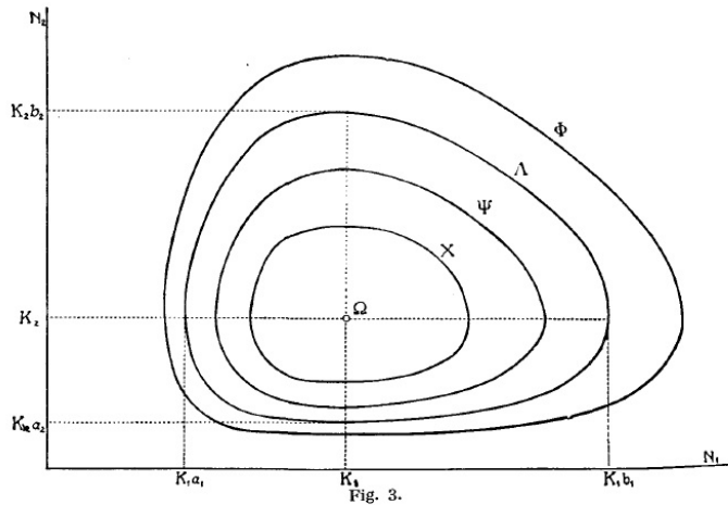
Figure 1: Periodic orbits in phase space. N_1 denotes the prey population; N_2 denotes the predator population. The orbits X , \Psi , \Lambda , \Phi are examples of the exhaustive and disjunct orbits corresponding to systems with different initial conditions. \Omega is the equilibrium state of all systems. If a system is not disturbed, it evolves on its orbit, running counter-clockwise with a constant period, and it stays on its orbit; this is Volterra’s “First Law”. Illustration from Volterra (1928, p. 14)
