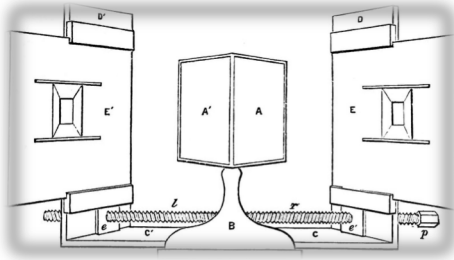
Figure 2. Wheatstone's stereoscope.
