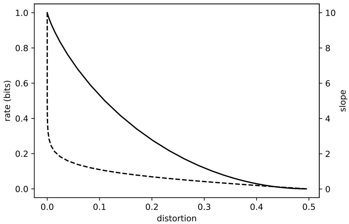
Figure 3: The rate-distortion function for a coin toss
