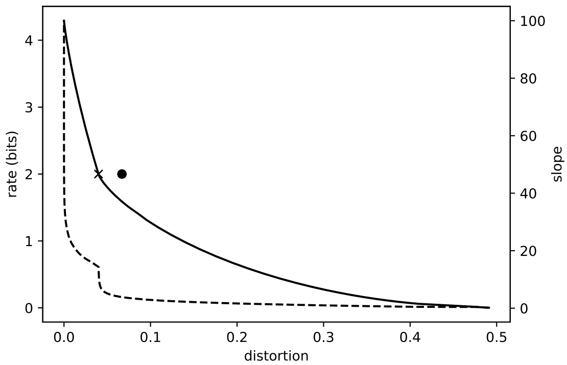
Figure 6: Cue-driven encoding
