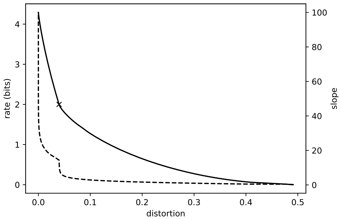
Figure 5: A sweet spot in the rate-distortion function
