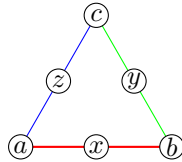
Figure 2: A “Greechie diagram” of the Wright Triangle, in which outcomes belonging to a common test lie along a smooth curve (here, a straight line).
