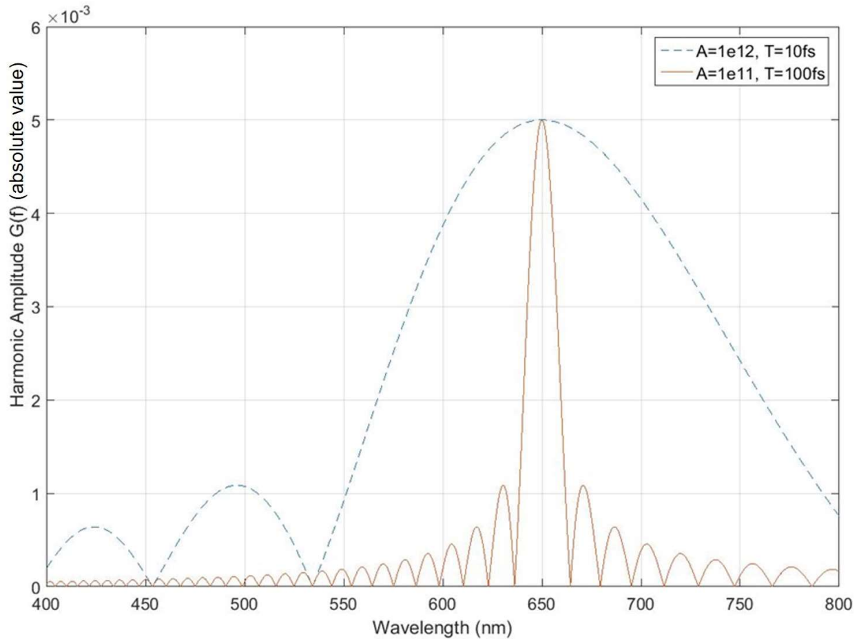
Figure 2: Fourier Decompositions of Short-Duration Pulses
