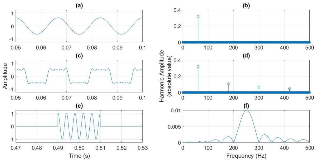
Figure 1: Superposition in the Time and Frequency Domains
