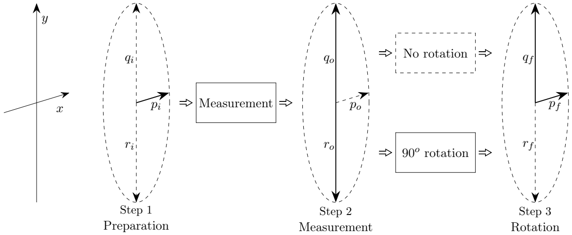
Figure 1: Graphic representation of the discussed example. Step 1 describes the preparation of the electron in the x -spin up state; Step 2 represents the measurement of S_y at a later time; finally in Step 3 we rotate the direction of spin by 90 degrees if at Step 2 the particle is found in the y -spin down state. We leave the direction of spin unchanged otherwise.
