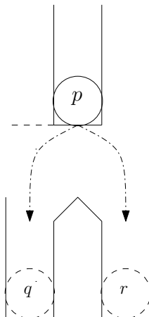
Figure 2: Graphic representation of the discussed example. Initially a ball is in position p over a hatch. After the hatch opens, the ball drops and falls to either position q or r with equal chance.
