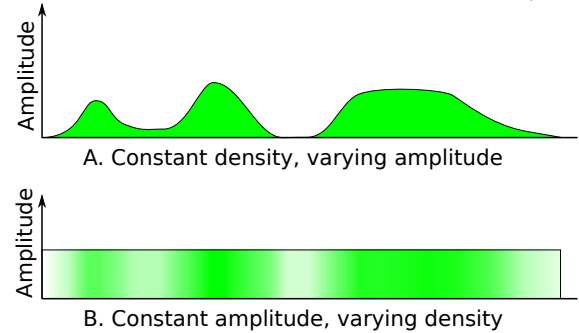
FIG. 1. The Born rule from counting basis states.
