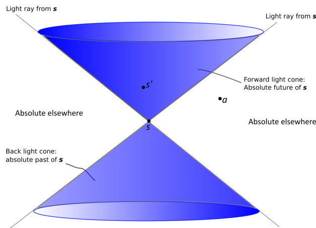
Figure 1: Relativistic spatiotemporal structures
