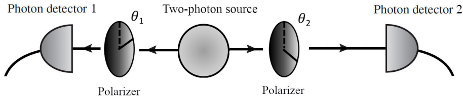
Fig. 1 Layout of an EPR-type experiment, in which entangled pairs of photons are sent in opposite directions by a two-photon source.
