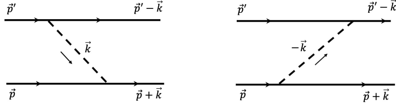
Fig. 4 Two processes for virtual phonon exchange between two electrons.
