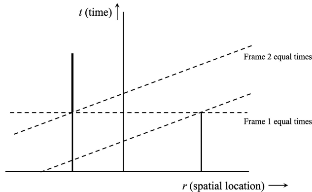
Fig. 3 World lines for a superposition of a fermion in two locations, with a collapse at some instant in time. The two thin vertical lines represent the two superpositions, each with half the total spectral weight, while the heavy vertical line on the left represents the state of the system after the collapse, in Frame 1, in which both states are at rest. From the perspective of the Frame 2, moving relative to Frame 1, the equal-time slices are given by the tilted dashed lines.
