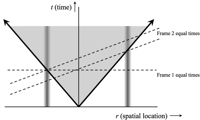
Fig. 2 World lines of the experiment of Figure 1, in the rest frame of the detectors. The vertical, fuzzy gray bars represent the world lines of the detectors; the solid black arrows give the world lines of the outgoing wave packets, and the gray area represents the causally-connected region of space time in which these two packets can be entangled. In this rest frame (Frame 1), a wave packet hits the detector on the left before the other wave packet hits the detector on the right. In a different frame of reference (Frame 2), this event occurs after the detector on the right encounters the wave packet.
