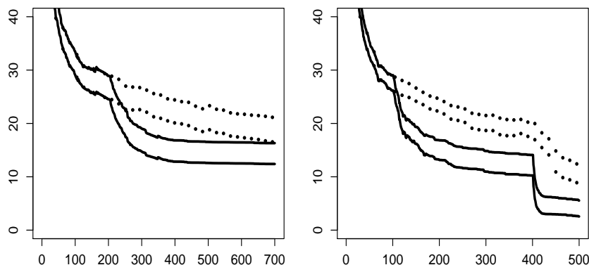
Figure 2: Confidence interval for best solution MSE by generation. Crossovers’ comparative performance: Standard (···) and SASC (—).
