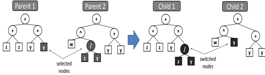
Figure 1: Example of destructive crossover
