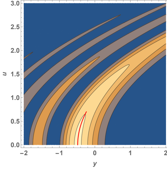
Figure 4: Contour plot, in the y - u plane with a = 0.1 , of the square of intensity of wavepacket (17) for the different lobes of the solution. The red line shows the deflection of this maximum intensity of this solution on this space.
