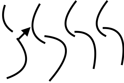
Figure 2: Discontinuous wave fronts for a generalised ‘wave’.
