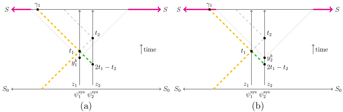
Figure 3.12. (a) highlights the part of S used to calculate the energy density at y_1^b whose time is greater than 2t_1 - t_2 . (b) highlights the part of S used to calculate the energy density at y_2^b whose time is greater than 2t_1 - t_2 .
