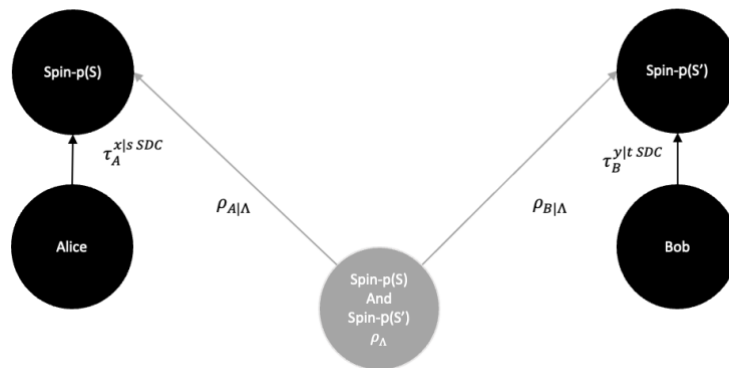
Figure 3: DAG of the common cause structure of Bell correlations, which respects relativity and is local, being represented by quantum causal models as interpreted by EnDQT.
