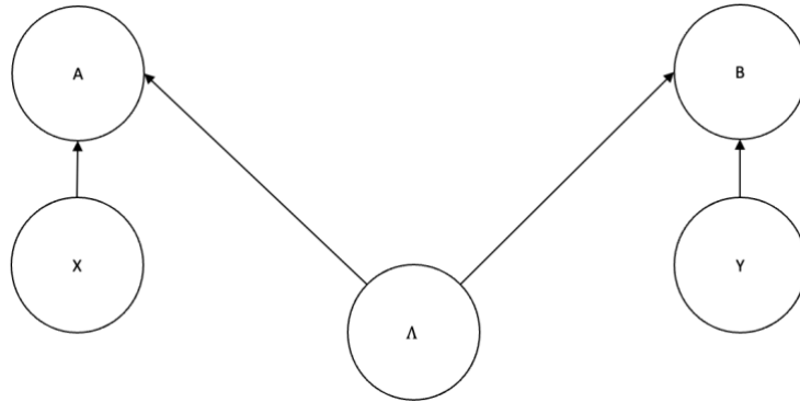
Figure 2: DAG of the common cause structure of Bell correlations, which respects relativity and is represented by classical causal models. This causal structure respects relativistic causality because X or A doesn't influence Y or B , and vice-versa, where these events may be spacelike separated, favoring a preferred reference frame. Moreover, no other variables influence the variables A , B , X , or Y , or they don't influence anything else. So, there are no so-called retrocausal or superdeterministic causal relations.
