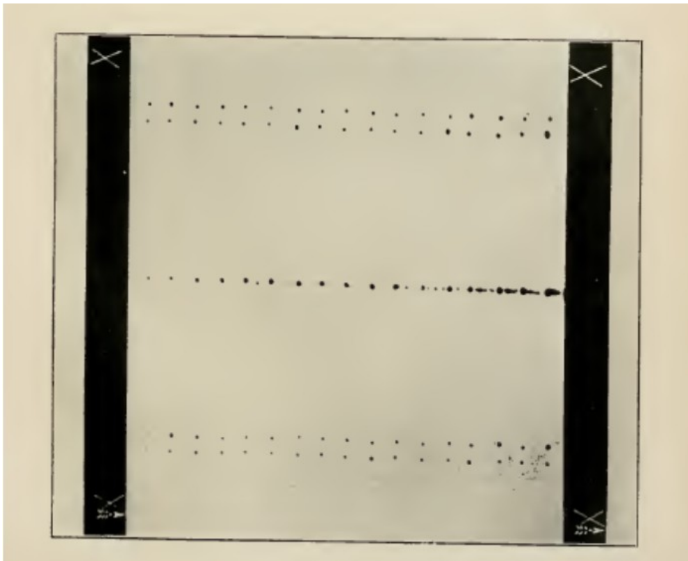
Figure 8: A negative of one of Guye and Lavanchy's photographic plates. 102
