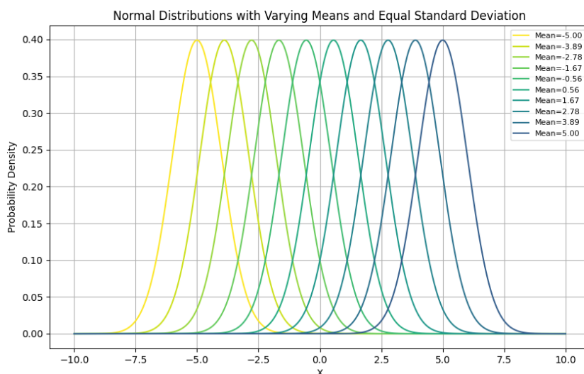
This is an accompanying graphic which demonstrates the presence of all possible linearly shifted normal distributions in the context of this particular mixed-decomposition of the normal distribution attribute.
