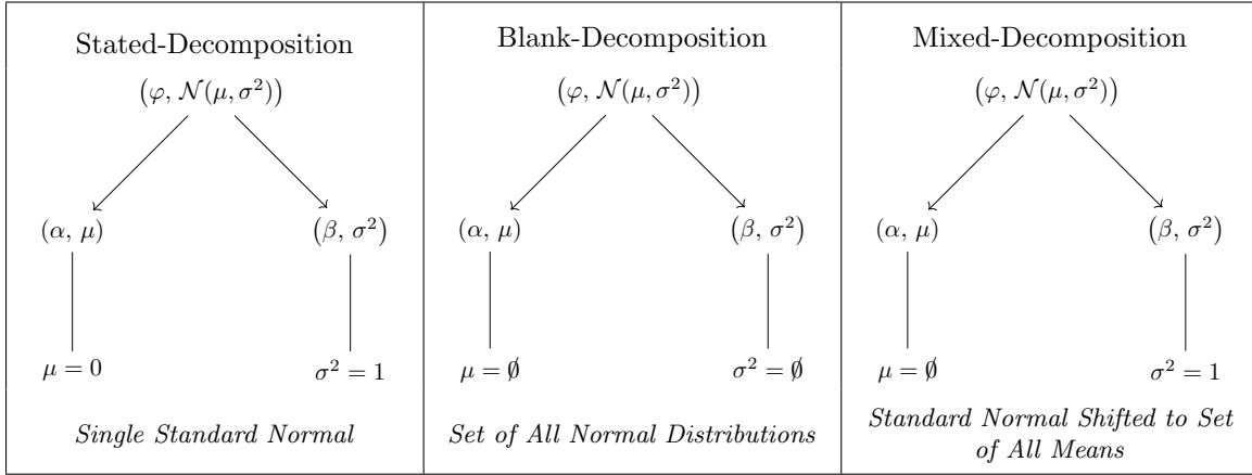
Figure 8: Shown above is an example with a normal distribution of the three major categories of an attribute’s presence in an Aethus, as well as what they represent when retrieved. A stated-decomposition means that the attribute has a single well-defined state in the \mathcal{B} -Aethus of that Aethus, a blank-decomposition means that the attribute is described in the \mathcal{B} -Aethus as blank, and a mixed decomposition means that the Aethus in question cannot be represented with the form of the attribute itself, as some of its component parts are stated while others are blank. [1]
