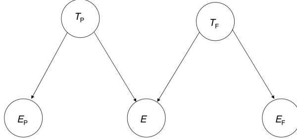
Figure 2: The Bayesian network representing the situation before the reduction.
