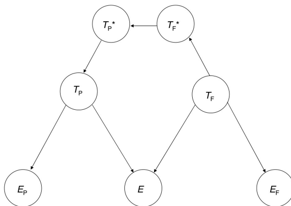
Figure 3: The Bayesian Network representing the situation after the reduction.
