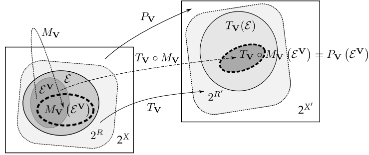
Figure 2: The relativity principle only implies that T_{\mathbf{V}} \circ M_{\mathbf{V}}(\mathcal{E}^{\mathbf{V}}) = P_{\mathbf{V}}(\mathcal{E}^{\mathbf{V}}) . Covariance of \mathcal{E} would require that T_{\mathbf{V}}(\mathcal{E}) = P_{\mathbf{V}}(\mathcal{E}) , which is generally not the case, except if M_{\mathbf{V}} : \mathcal{E}^{\mathbf{V}} \rightarrow \mathcal{E} is surjective
