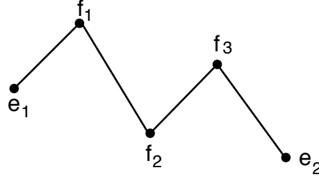
Figure 2: A snake-link between e_1 and e_2 .
