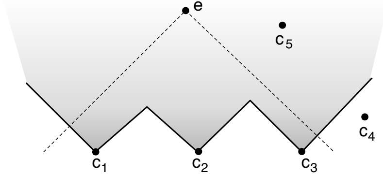
Figure 3: Illustrating the sets W_e^C . c_1 , c_2 and c_3 are the choice events in e 's causal past indicated by the dashed lines ( c_4 and c_5 are outside that region). The region W_e^C is shaded grey; the boundary is not part of W_e^C . Note that W_e^C contains all events above c_5 , even though events in different continuations of c_5 are incompatible.
