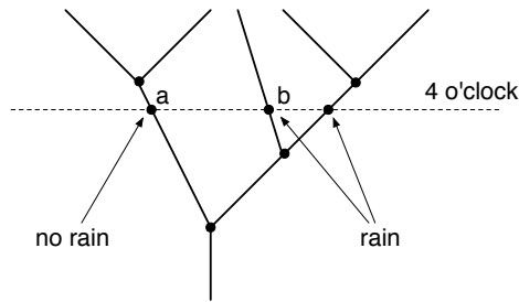
Figure 1: A branching tree of possibilities: rain or no rain at 4 o’clock.
