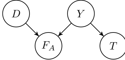
Figure 2: The Bayesian Network representation of the four-propositions scenario.
